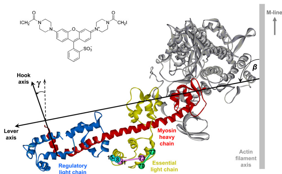
FIGURE 1 Ribbon representation of the head region of chicken skeletal myosin in the nucleotide-free state (PDB 2mys; (1)) bound to an actin filament in the absence of ATP (2), showing the lever and hook axes, and the tilt ( \beta ) and twist ( \gamma ) angles. Pairs of cysteine residues introduced into the ELC and cross-linked using BSR-I 2 (inset) are shown as spheres joined by rods.
